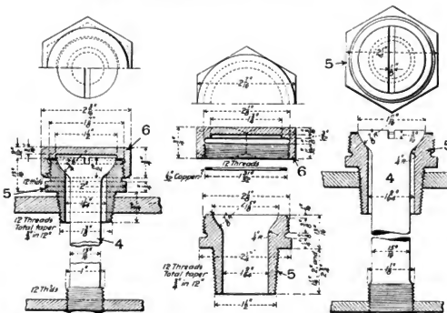
Figs. 298-305. Flexible Staybolts. Pennsylvania Railroad.
